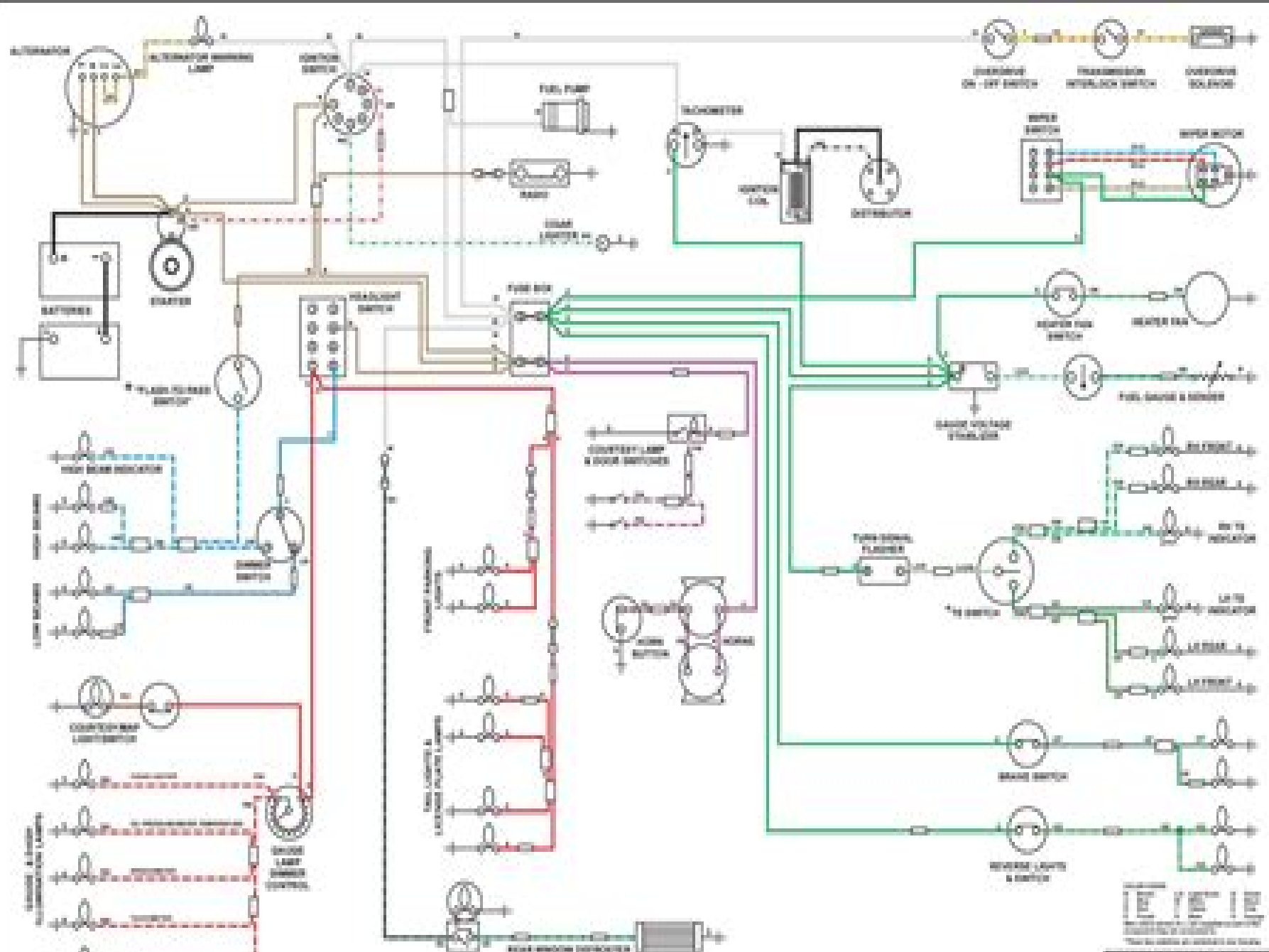
DIAGRAM 4 - 1988 MGB FROM BENTLEY B2330W
