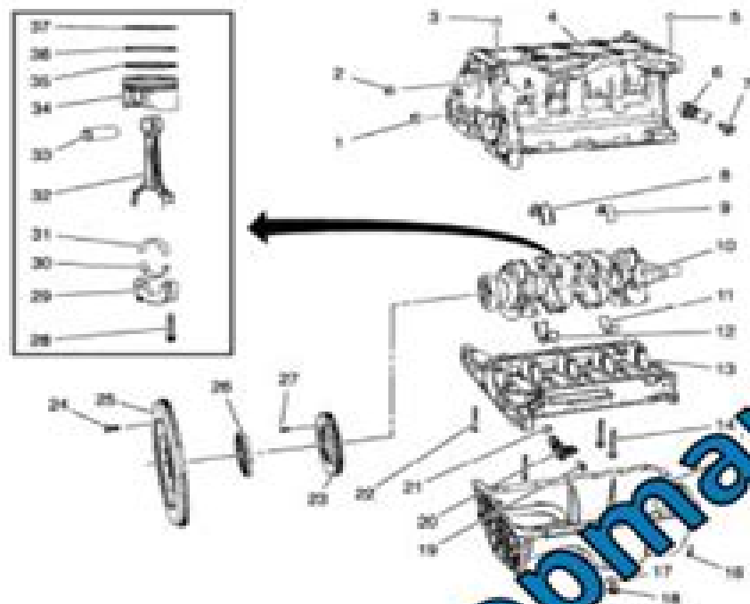
Fig. 7. Identifying Engine Block Assembly Components Courtesy of GENERAL MOTORS CORPORATION
