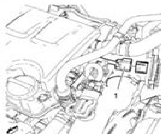
Fig. 9. Remove Oil Pan
