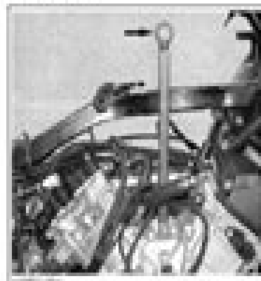
ATTACH THE ENGINE LIFTING TOOL FROM THE BOTTOM
