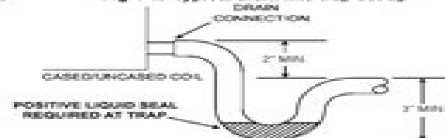
Fig 4-1. Typical drain line trap set up
