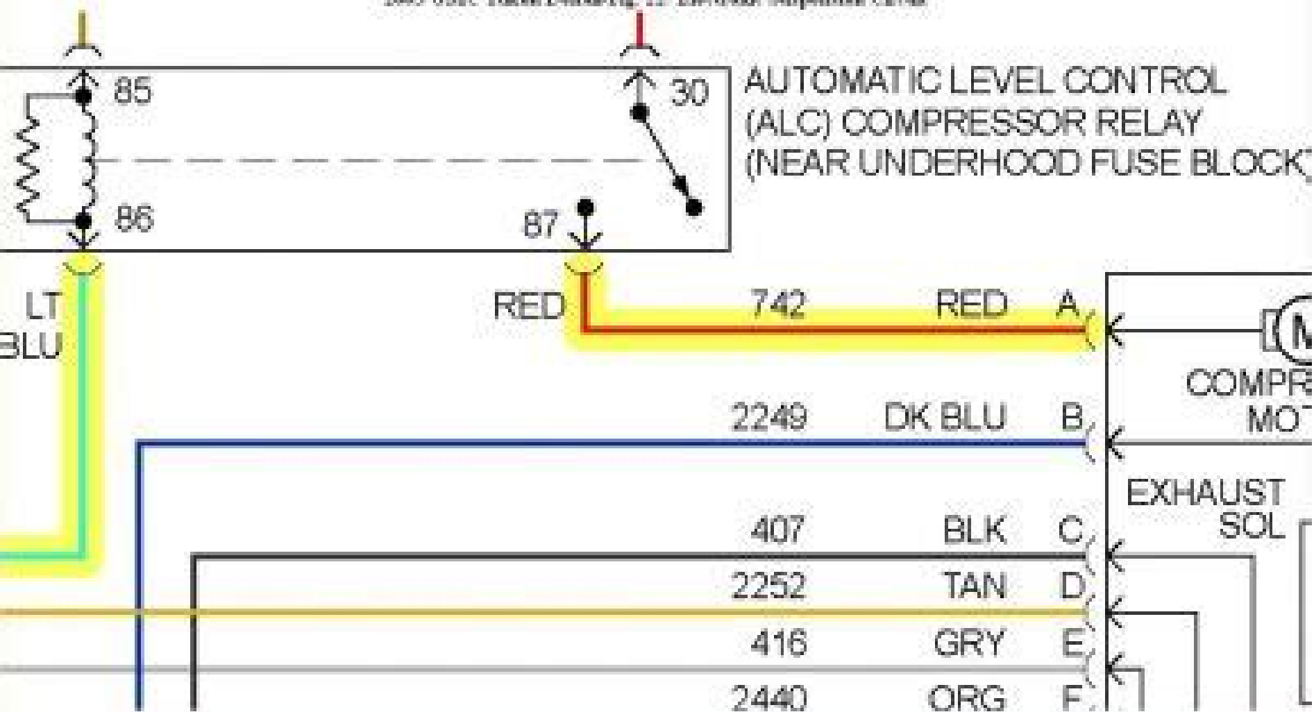
2003 GMC Token Dash-Fig. 11: Electronic Suspension Circuit
