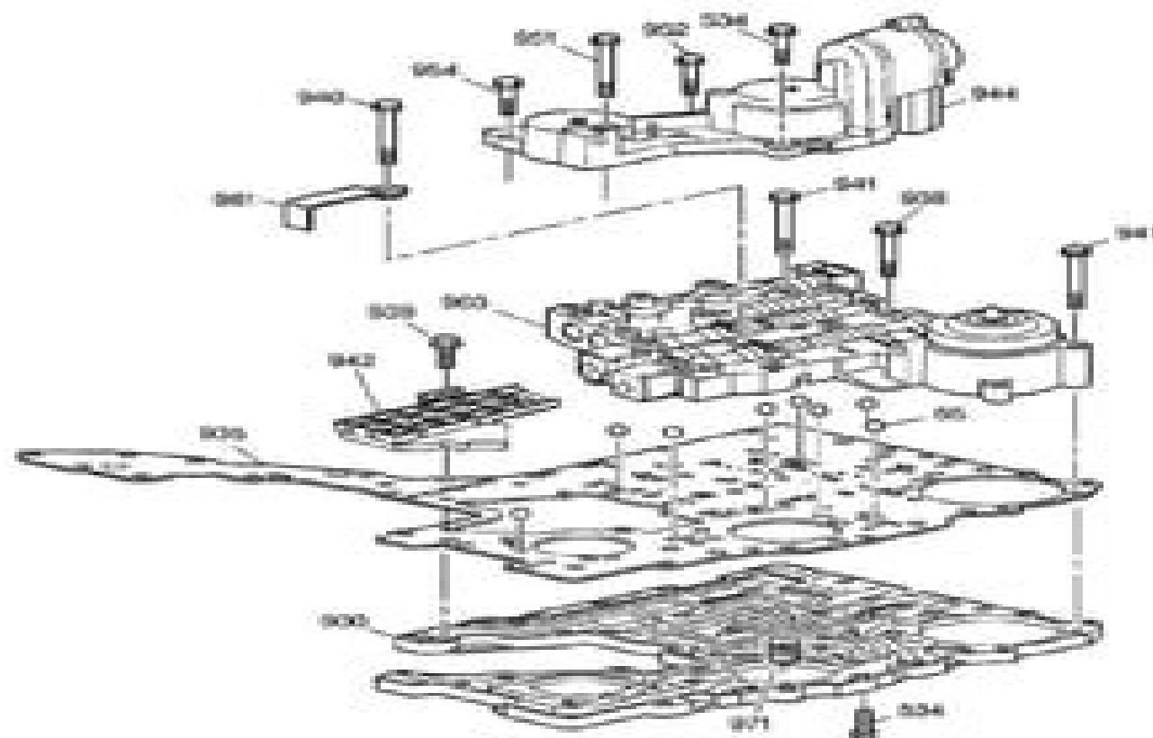
Fig. 6: Lower Channel Plate, Control Valve Body and Accumulator Housing Assembly Disassembled View Courtesy of GENERAL MOTORS CORP.
