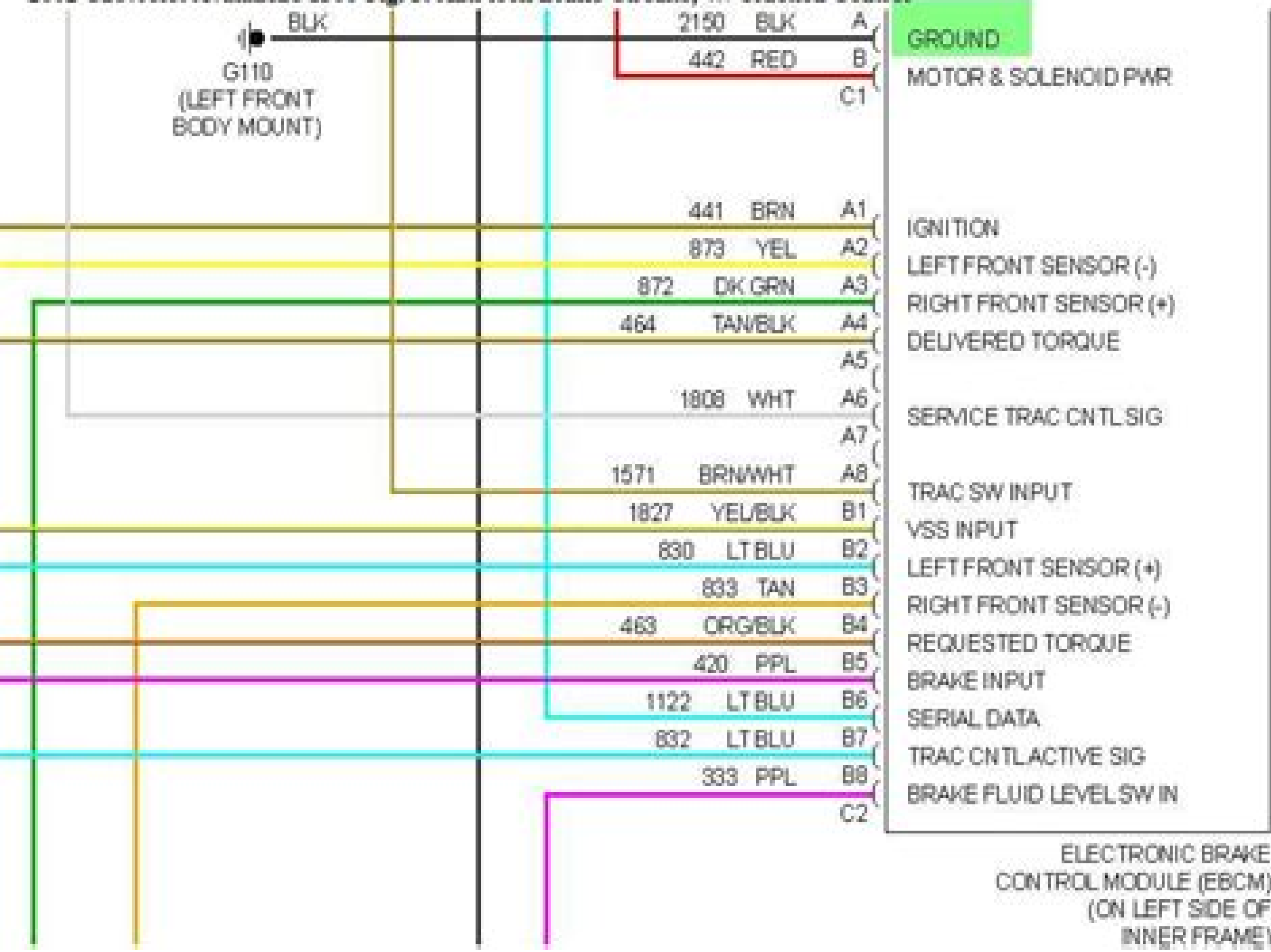
2002 Chevrolet Avalanche 1500-Fig. 5: Anti-lock Brake Circuits, W/ Traction Control
