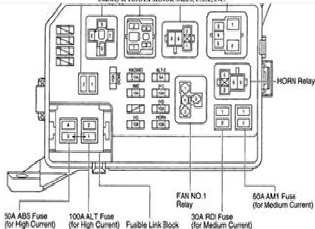
Fig. 10: Identifying Engine Room J/B Components Courtesy of TOYOTA MOTOR SALES, U.S.A., INC.
