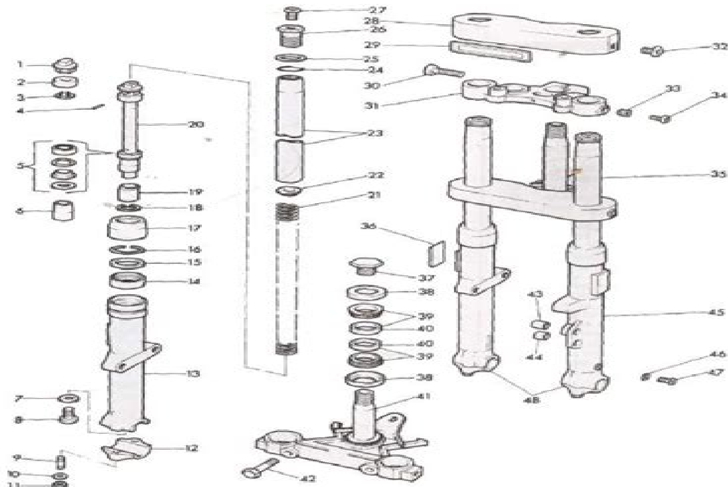
Typical FX model fork components
