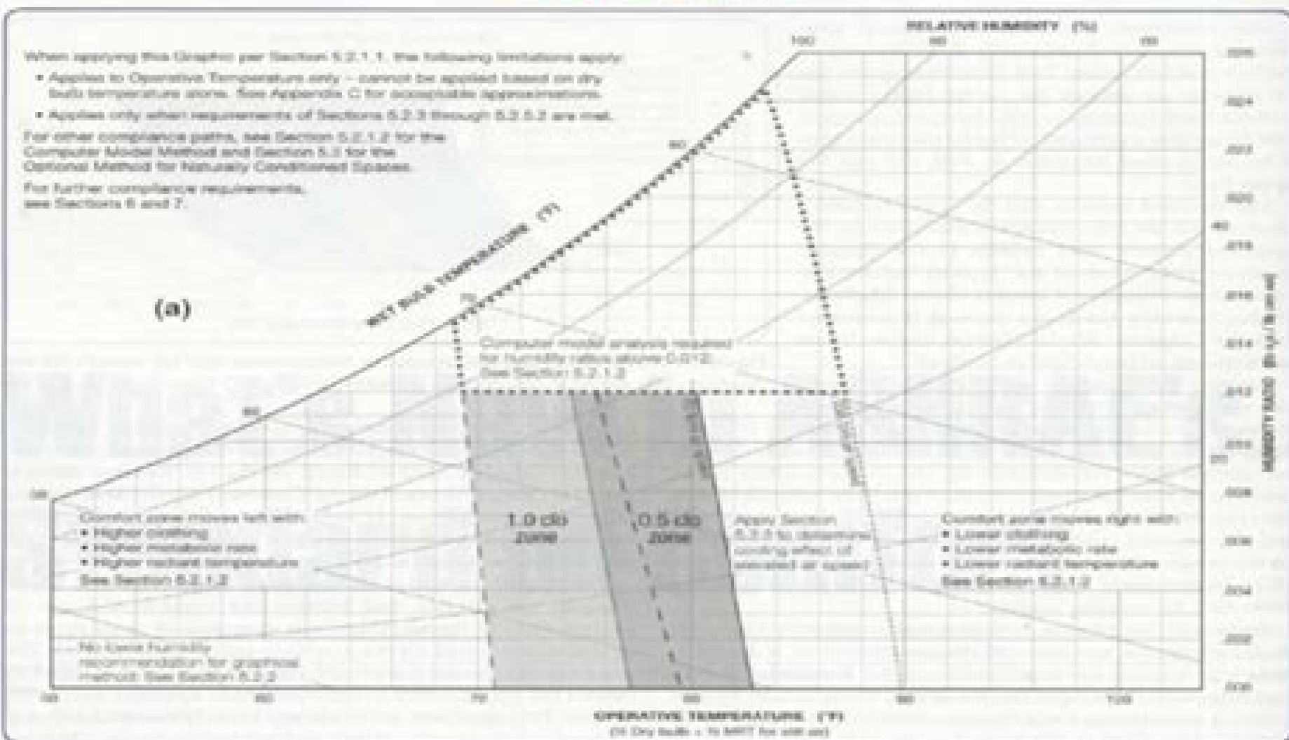
Figure 2: The new Graphic Comfort Zone Method, Figure 5.2.1.1 in Standard 55-2010 (IP version shown).
