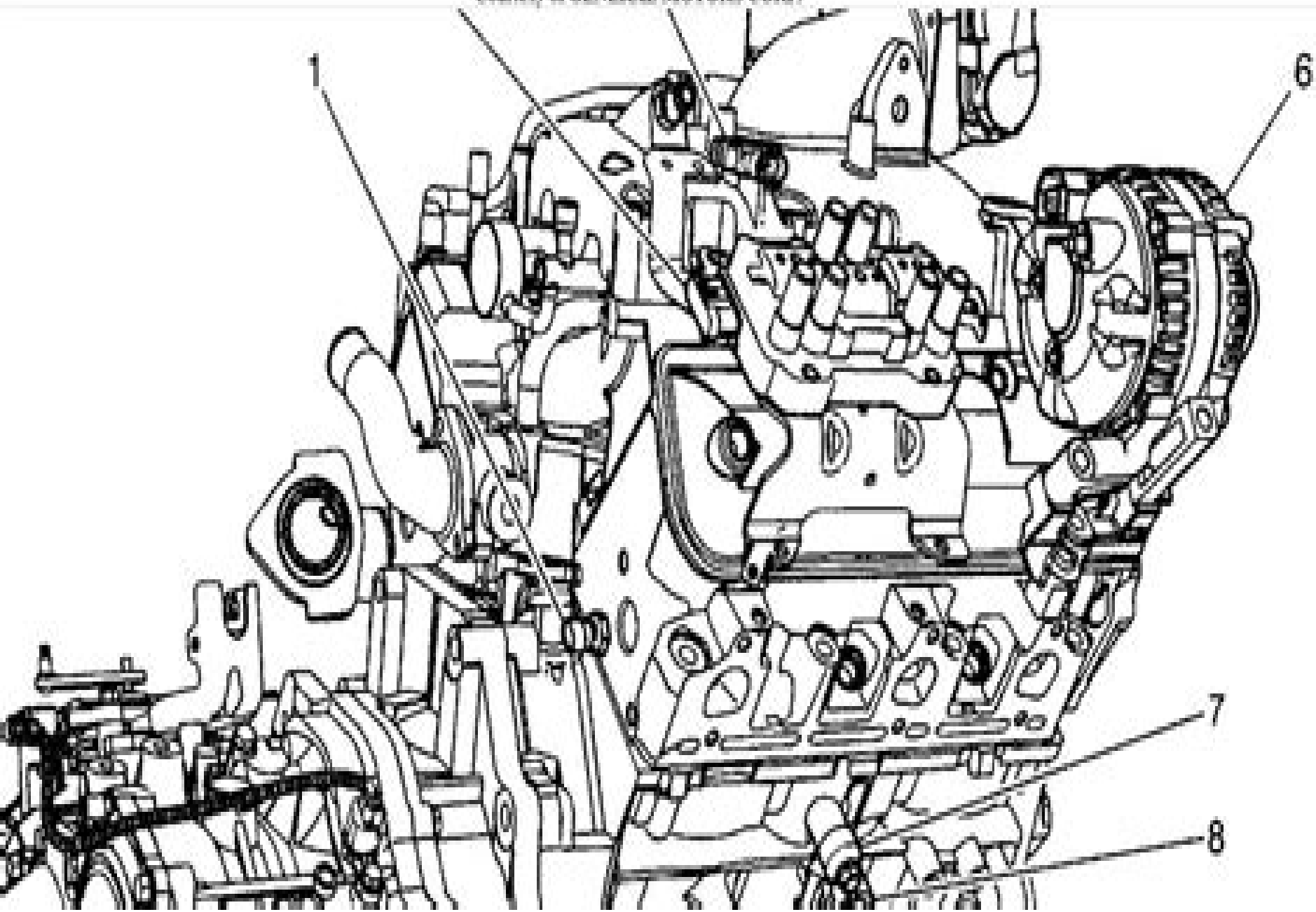
Fig. 22: Rear Of Engine
