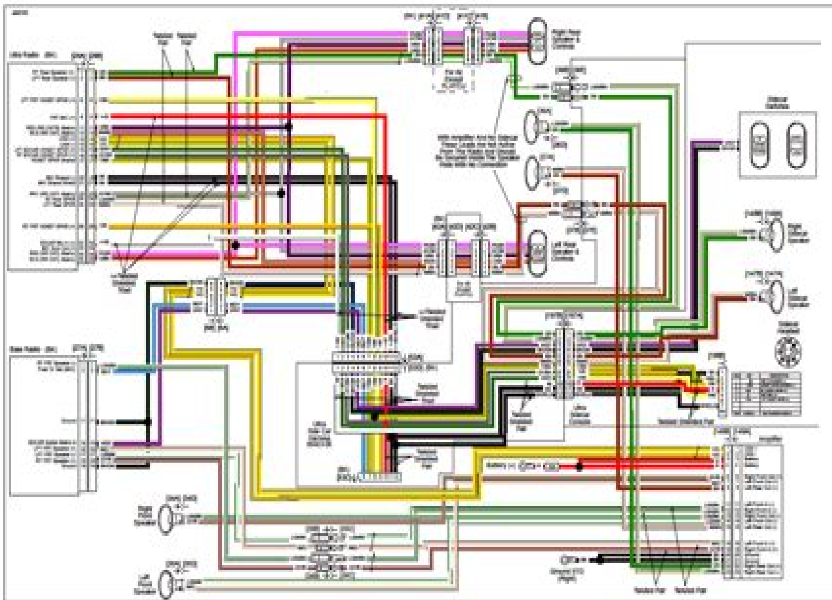
Figure 6-10 2000 Commodore Ultra-Radix Circuit
