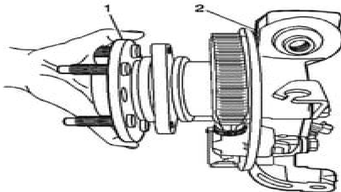
Fig. 4: View Of Wheel Bearing/Hub Assembly & The Knuckle Courtesy of GENERAL MOTORS CORP.
