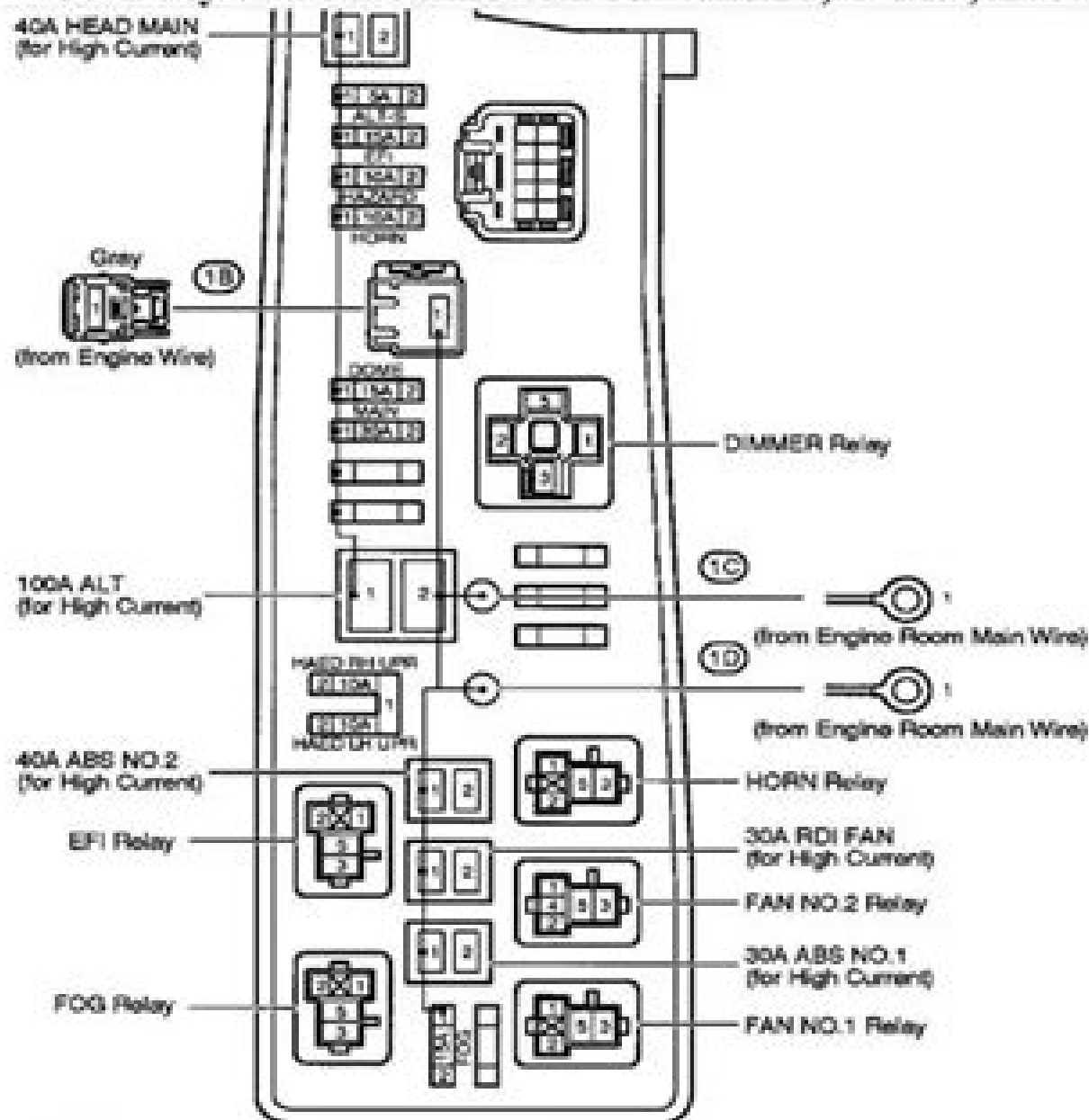
Fig. 3: Identifying Engine Compartment Junction & Relay Block Components
