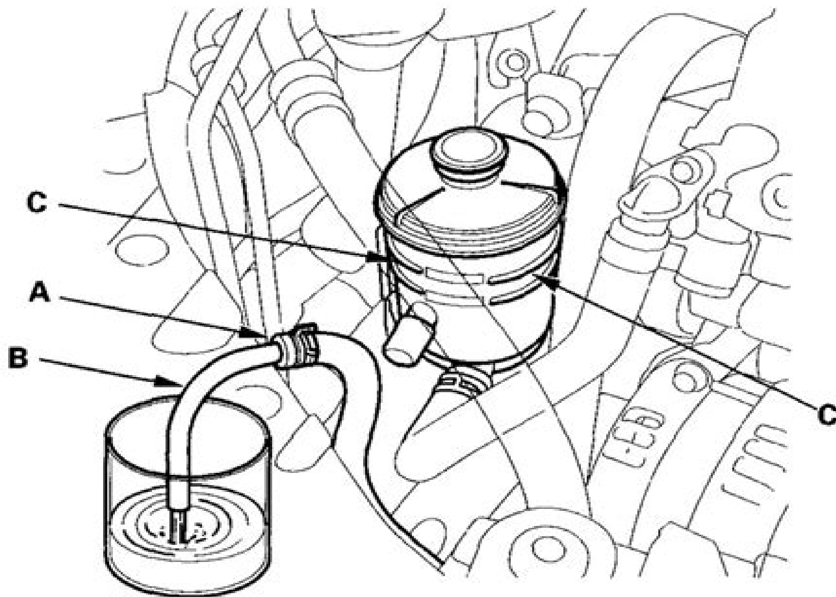
Fig. 12: Disconnecting Return Hose (A) To Drain Reservoir Courtesy of AMERICAN HONDA MOTOR CO., INC.
