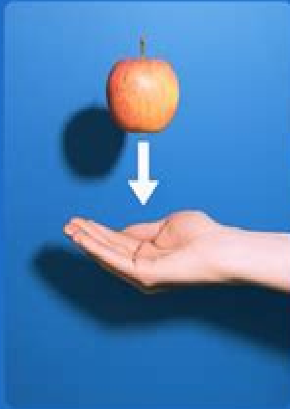
Gravity
