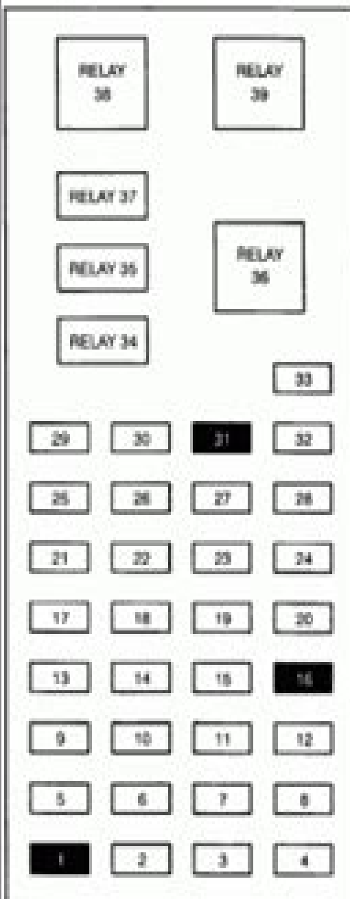
I/P FUSE PANEL
