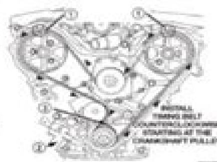
Fig. 78 Timing Belt-Installation
