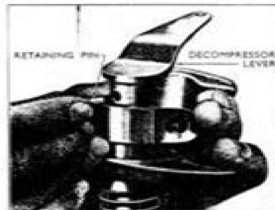
Fig. 3 Decompressor Lever
