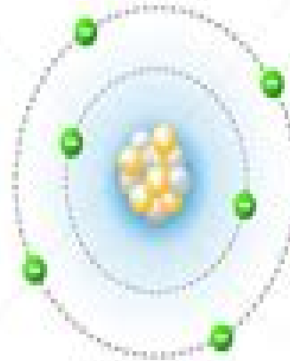
Bohr model
