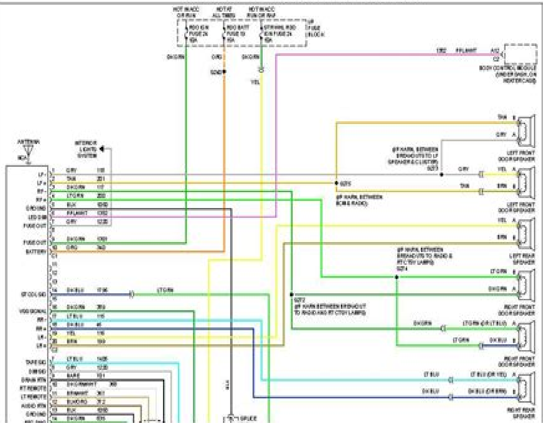
2001 GMC Jimmy - Fig. 49: Radio Circuits, W/O Amplifier
