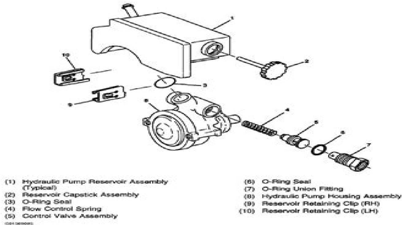
Fig. 5: Exploded View Of Power Steering Pump Assembly-CB Series Courtesy of GENERAL MOTORS CORP.
