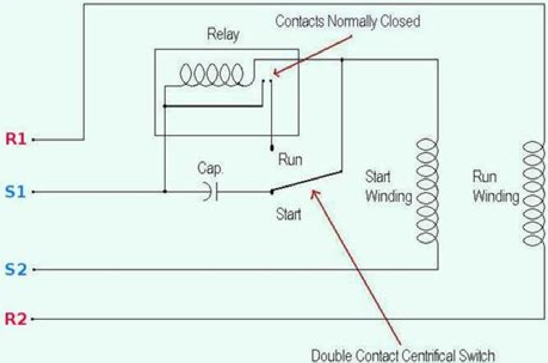
Four Lead Instant Reversing Single Phase Motor
