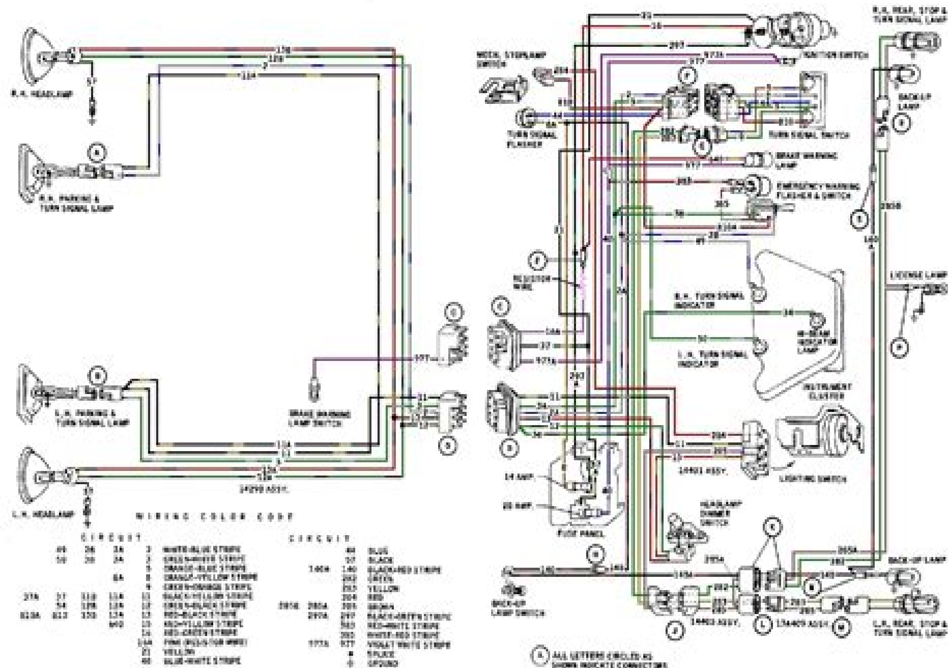
Wiring diagram for the exterior lights and turn signals—1967 Broncos
