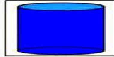
Cylinder
