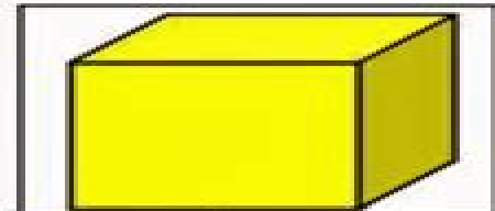
Cube
