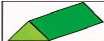
Triangular Prisms
