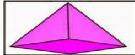
Square Pyramid
