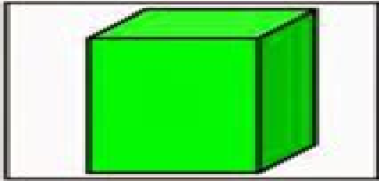
Rectangular Prism
