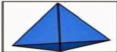
Triangular Pyramid
