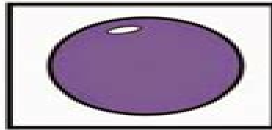
Sphere
