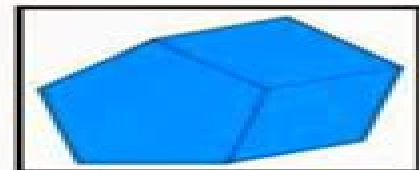
Pentagonal Prism
