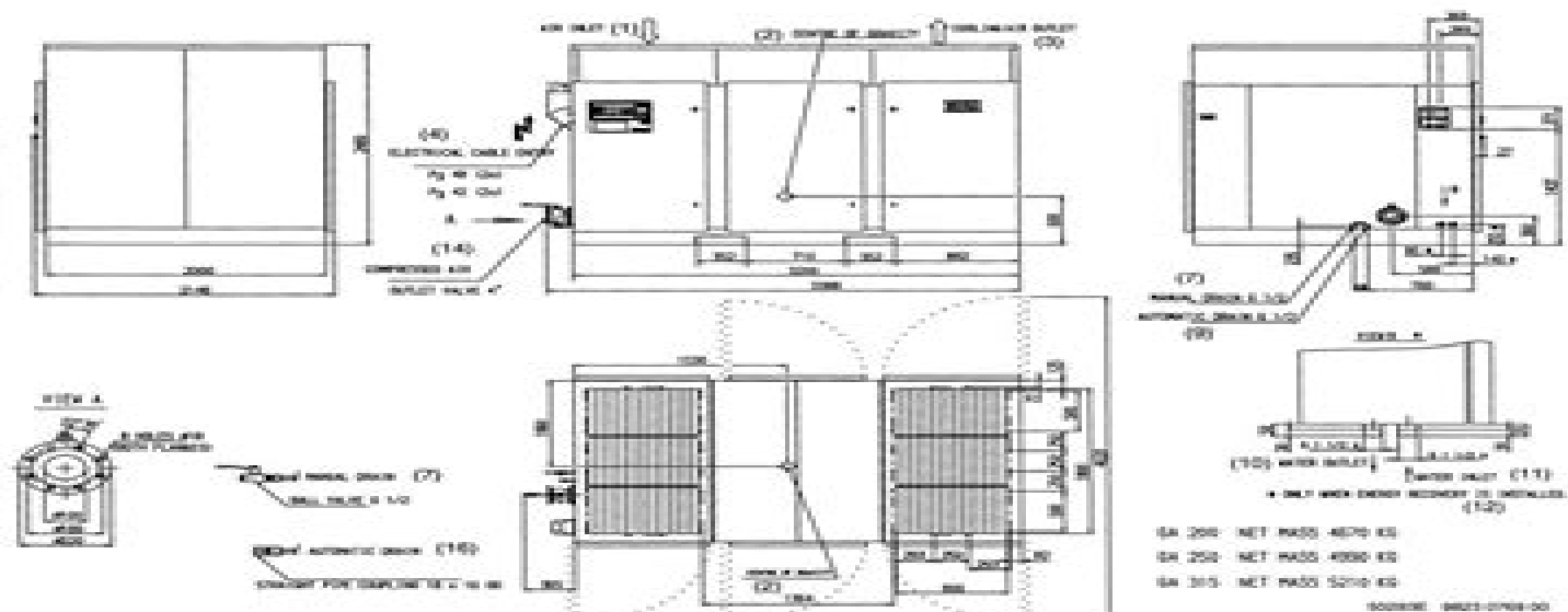
Fig. 6e. Dimension drawing GA200 up to -315
