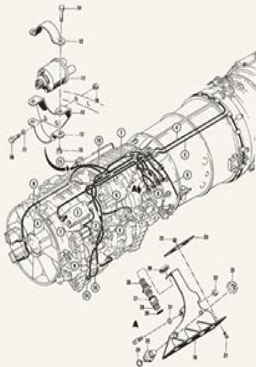
FIGURE 35. ELECTRICAL SYSTEM (Continued) (From 1 of 2 Views)
