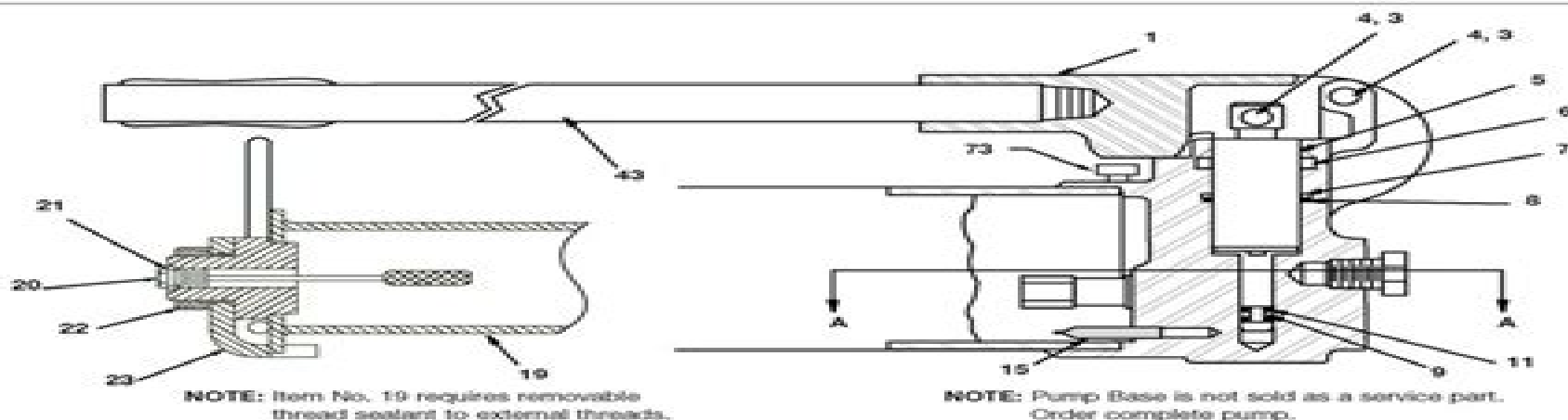
Figure 1, Pump Assembly
