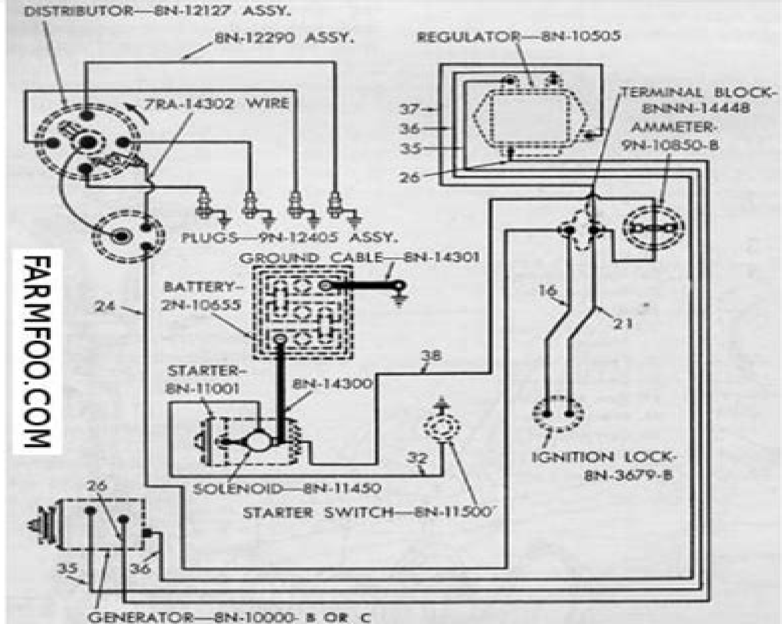
Fig. F043A - Schematic wiring diagram used on 8N tractors (with 2 brush generators and angle drive distributors) after tractor serial 263844.
