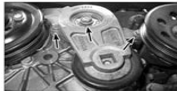
24.25 Typical V8 tensioner mounting fastener locations
