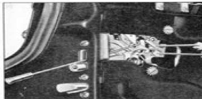
Fig. 35—Removing Lock from "Free-Wheeling"
