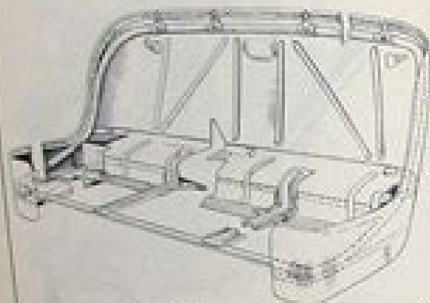
Figure No. 122 Section front seat metal rail frame.
