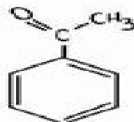
Acetofenone
