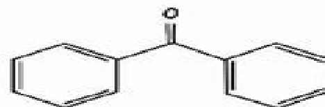
Benzofenone
