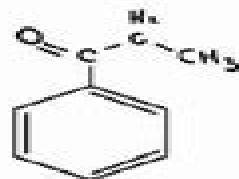
Propiofenone
