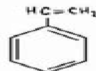
Stirene
