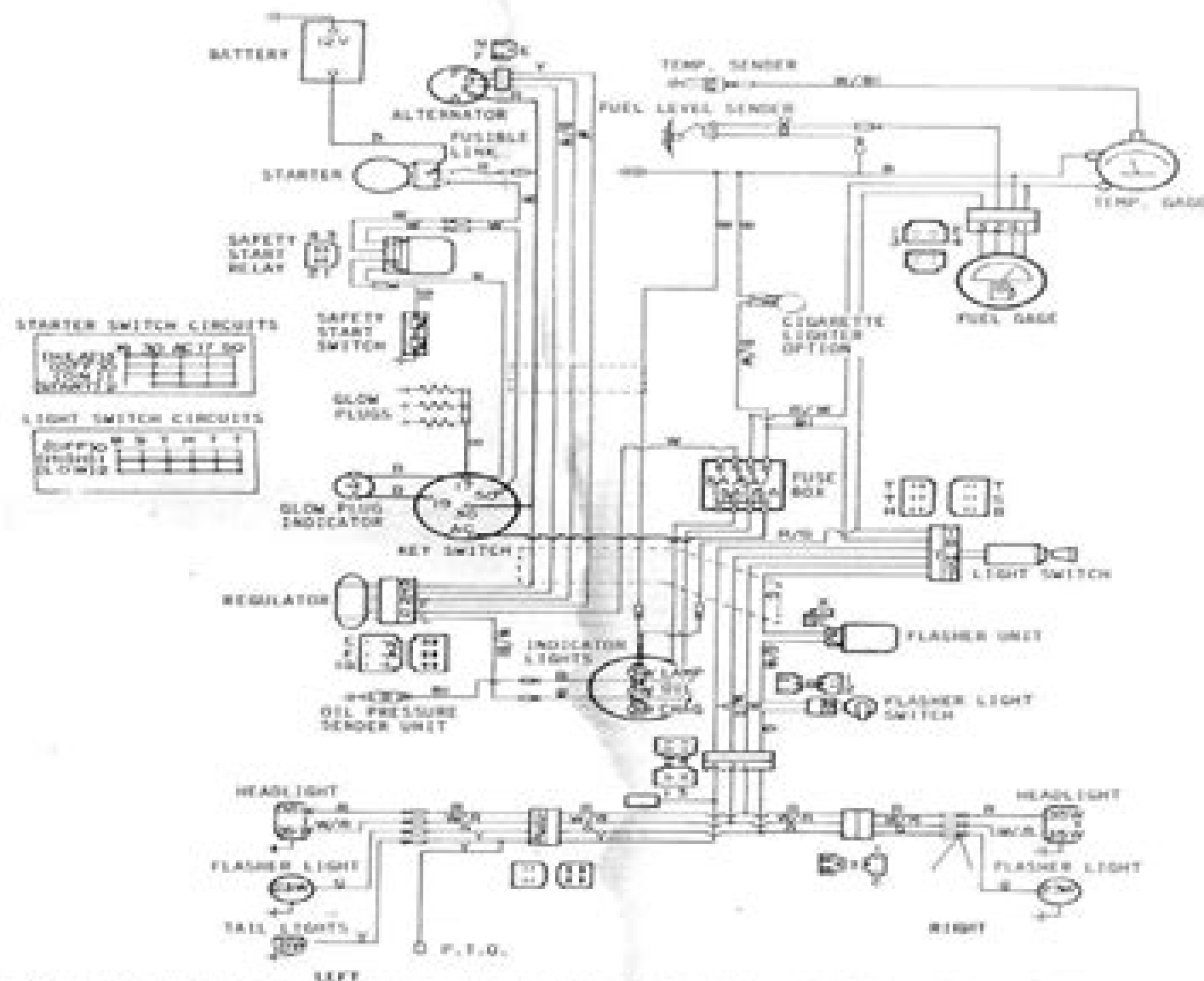
Fig. 387—Wiring diagram typical of late production (July 1965 and after) 1710 models. Refer to Fig. 386 for wire color code.
