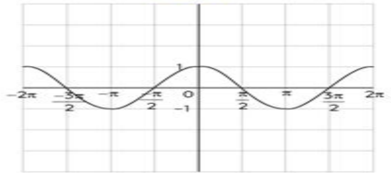
\cos\theta
