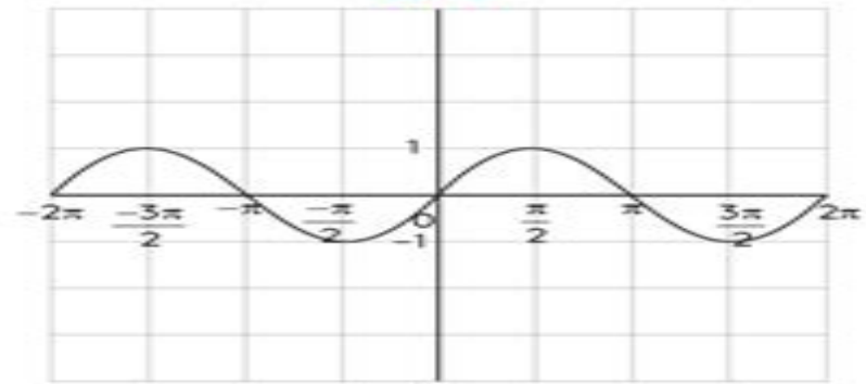
\sin\theta
