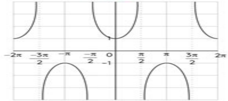
\sec\theta
