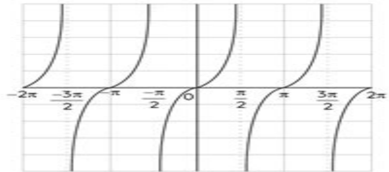
\tan\theta
