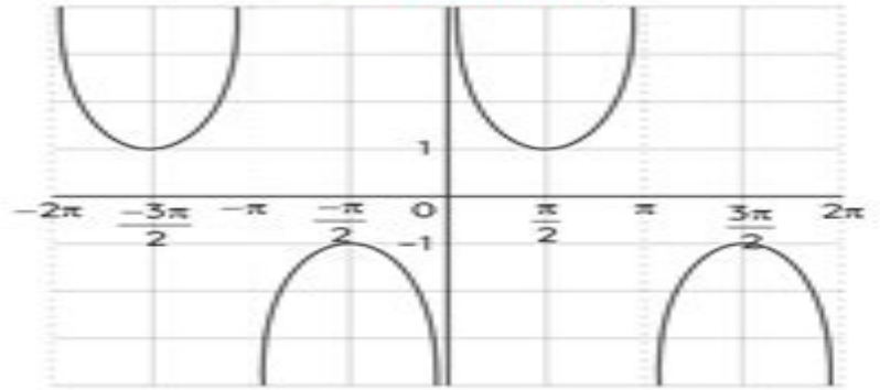
\operatorname{cosec}\theta
