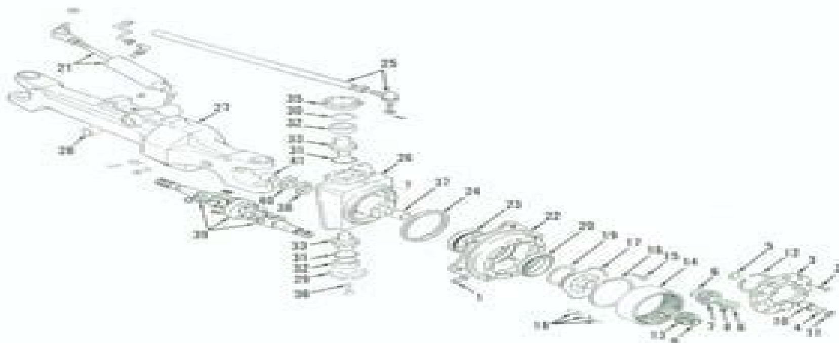
Fig. 14—Exploded view of front-wheel drive steering knuckle and planetary assembly.
