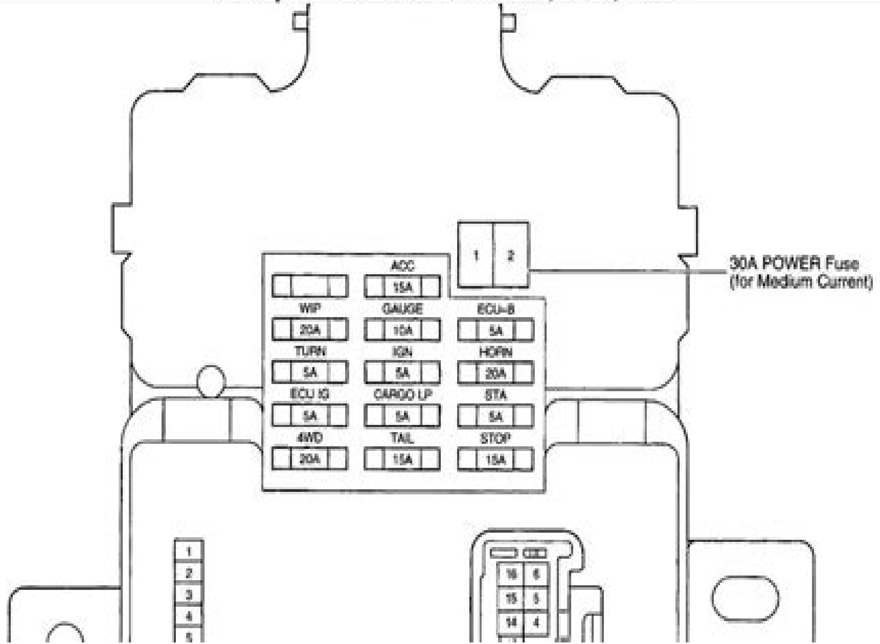
Fig. 2: Identifying Driver Side J/B & Integration Relay Components
