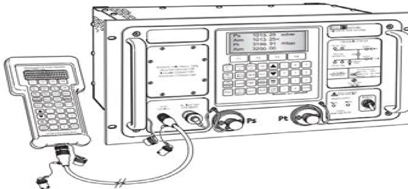
FIGURE 1-1 ADTS 405 GENERAL VIEW
