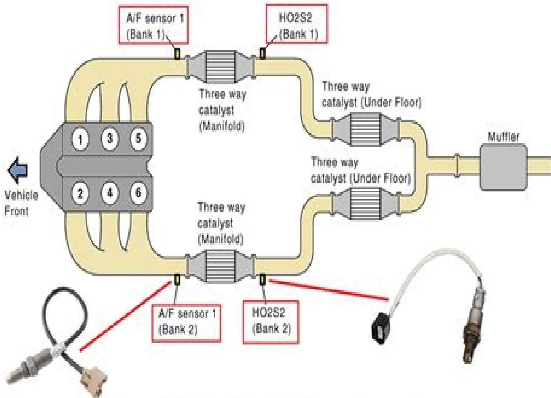
Nissan Pathfinder Air/Fuel Ratio Sensor - Oxygen Sensor
