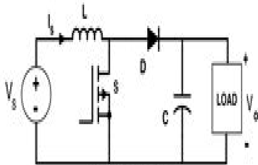
Boost Converter
