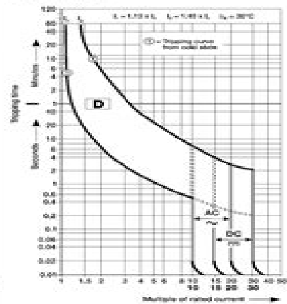
D characteristic
