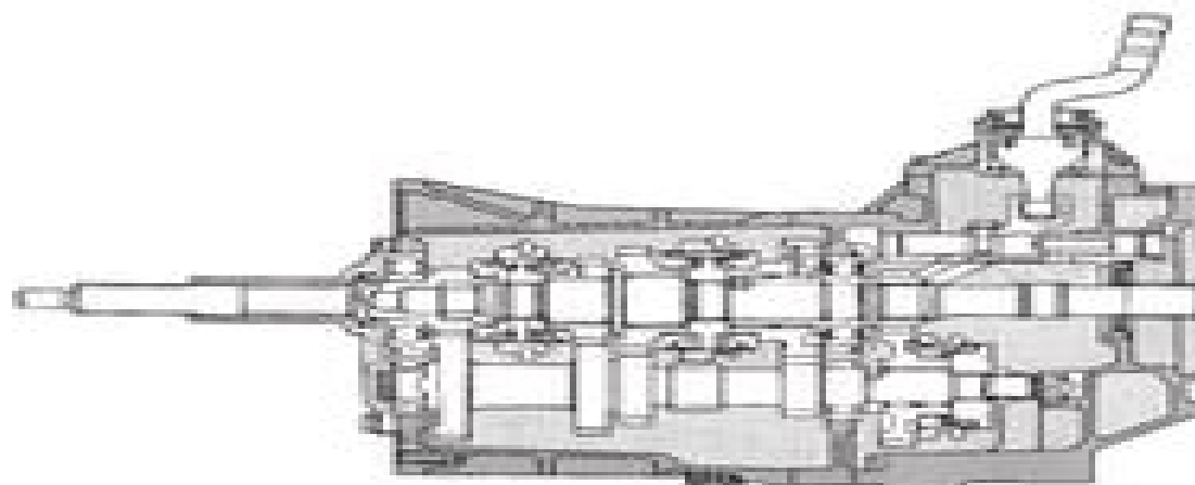
Fig. 1 AX 4/5 Manual Transmission
