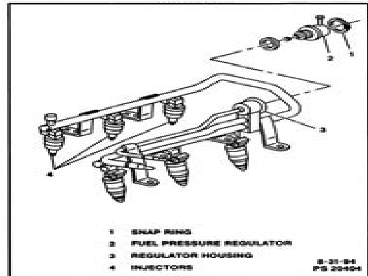
Figure C2-8 - Fuel Pressure Regulator Service
