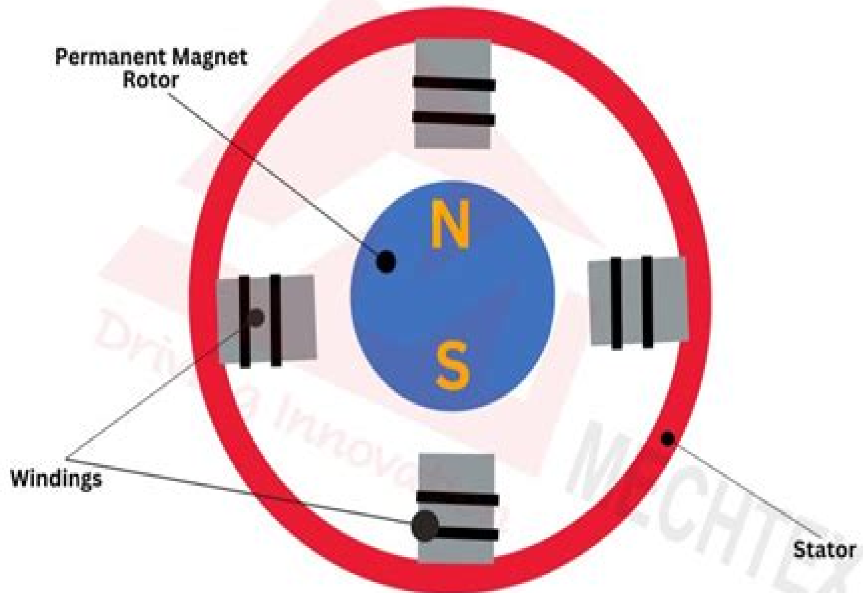
Synchronous Motor
