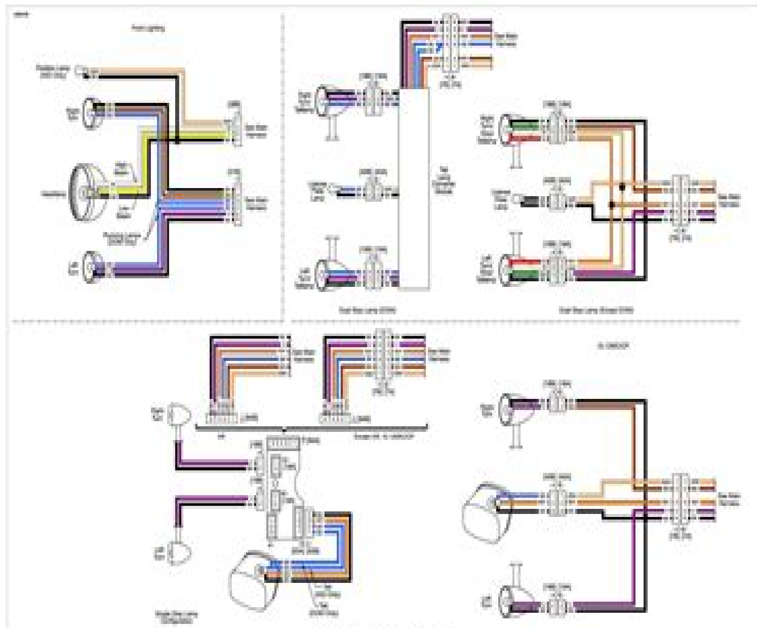
Figure 8-11: Lighting (Continued) - 2014 Edition
