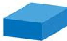
CUBOID
