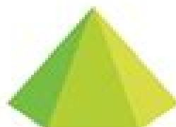
HEXAGONAL PYRAMID
