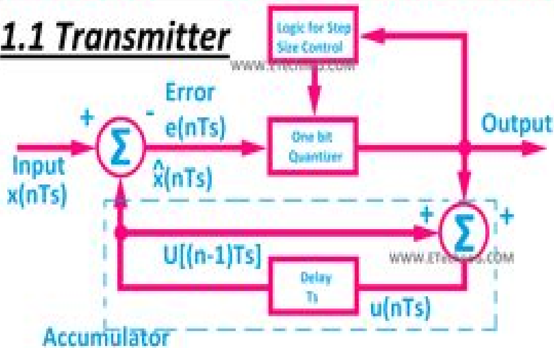
Figure.01: Adaptive Delta Modulation Block Diagram
