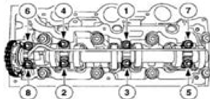
Fig. 422. Tightening Bolts in Sequence.
