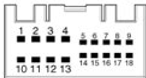
Connector A
