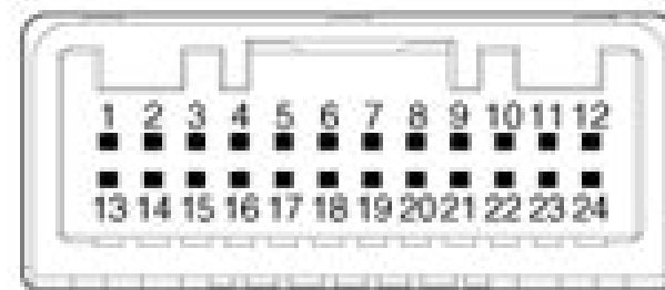
Connector C
