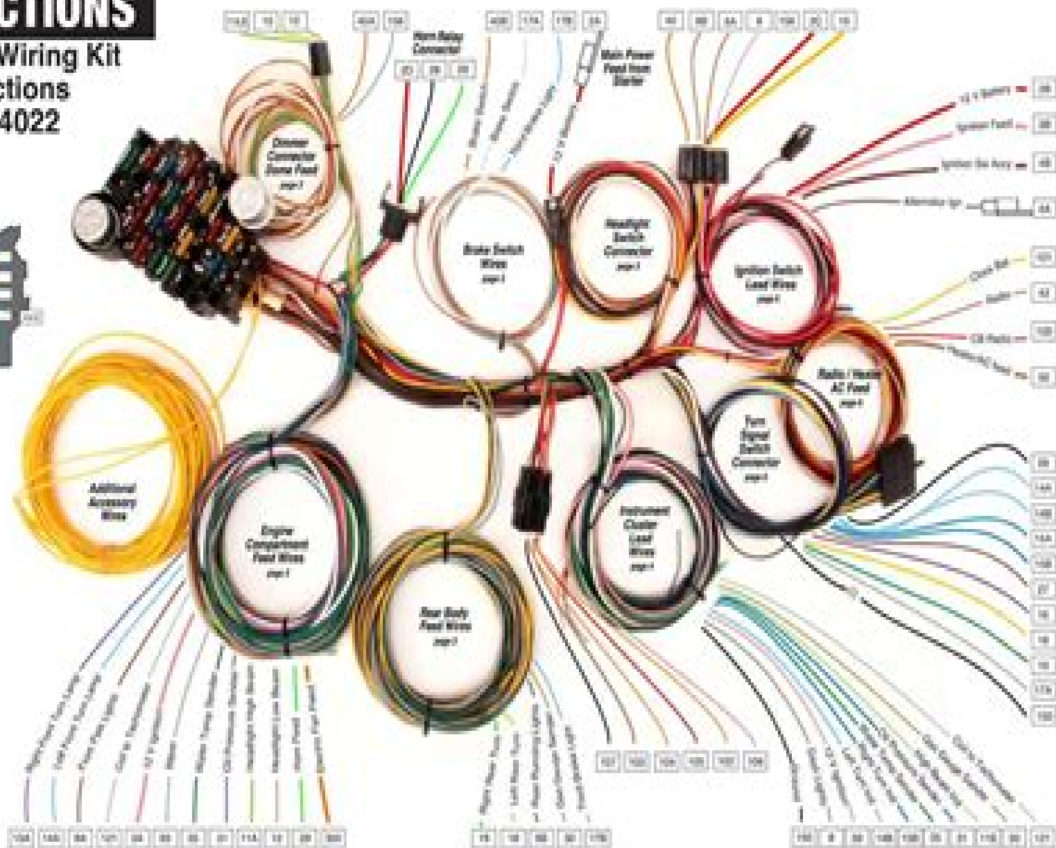
Fuse Box Connections (Connect both ends)
